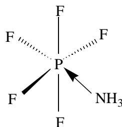
Pentafluorophosphorane-ammonia adduct/complex
