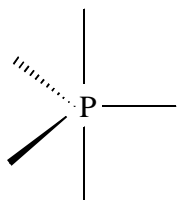
TrigonalBiPyramid (TBP)
