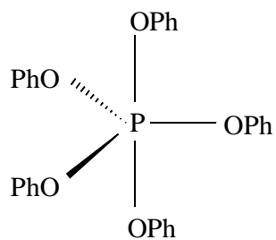
Pentaphenoxy phosphorane
