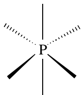
Octahedral (Oh)
